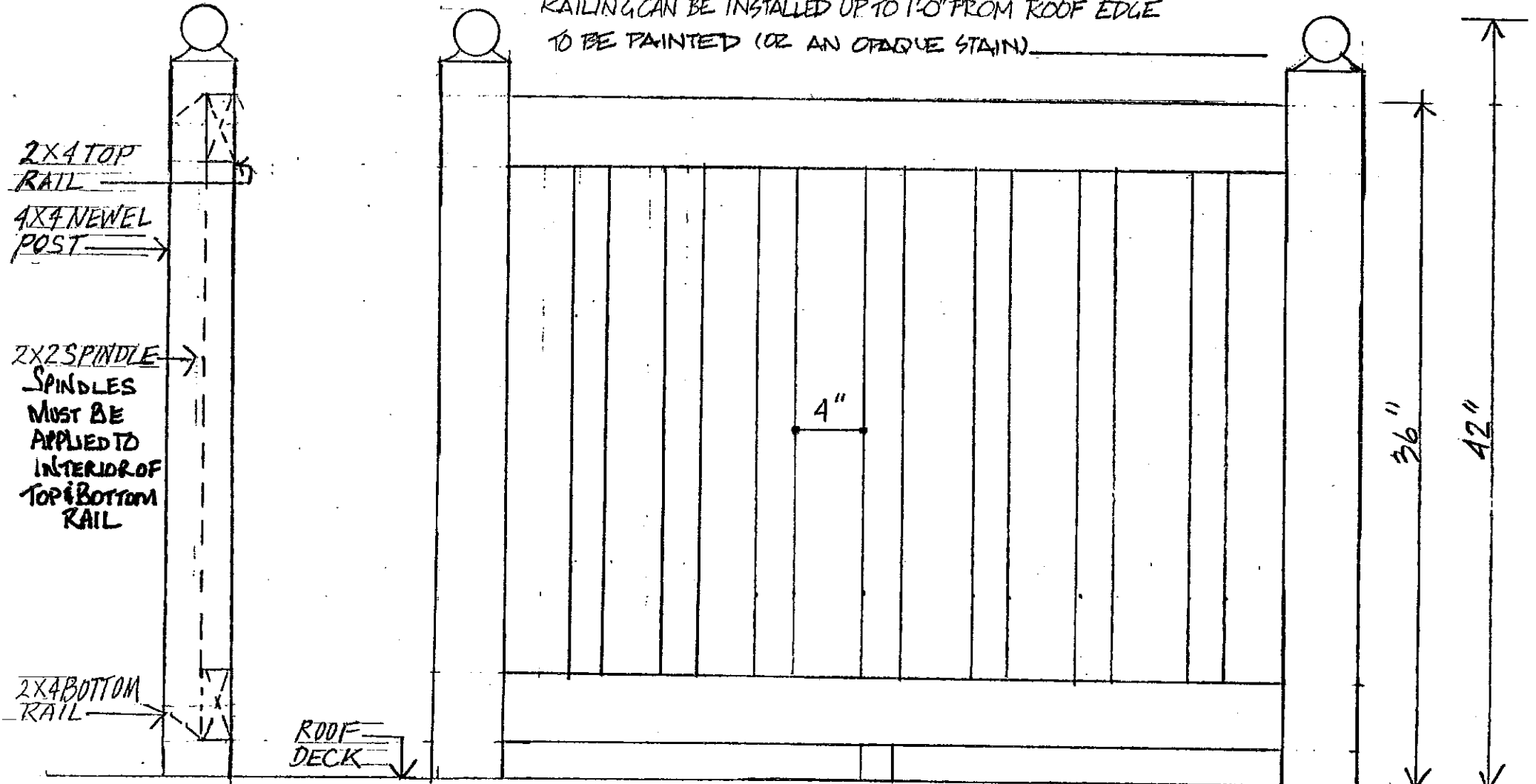
SECTION VIEW
