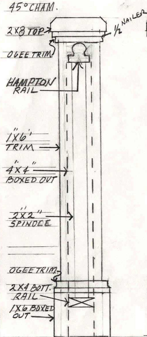
SECTION VIEW
